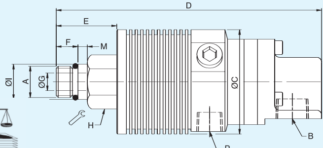
Radial Connection
