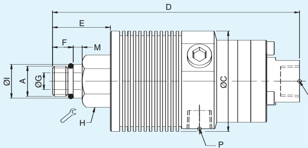
Axial Connection
