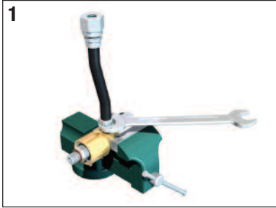
1 Mount housing in a bench vise and install hose.
